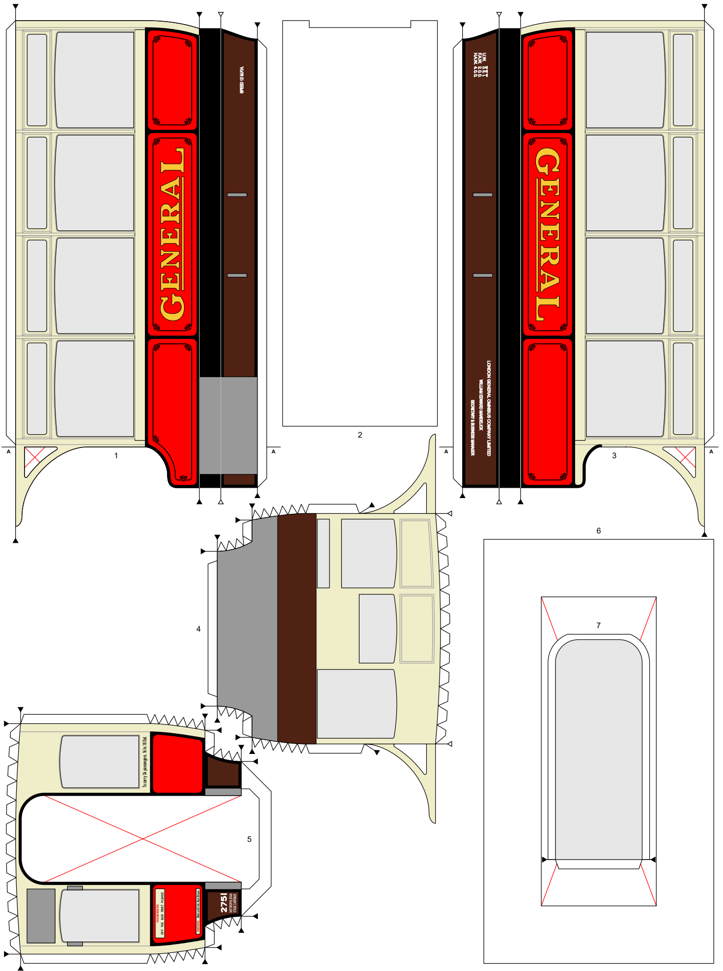
B-TYPE LONDON BUS 1:32 B: LOWER DECK SIMPLE - B1 -
